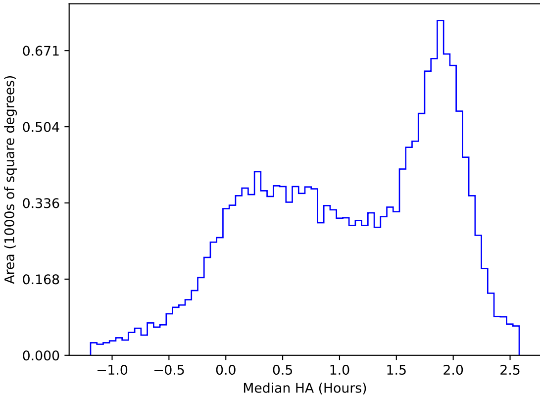
internal_u_expt45_nscale0.9v3.4_10yrs WFD u band: Median HA
