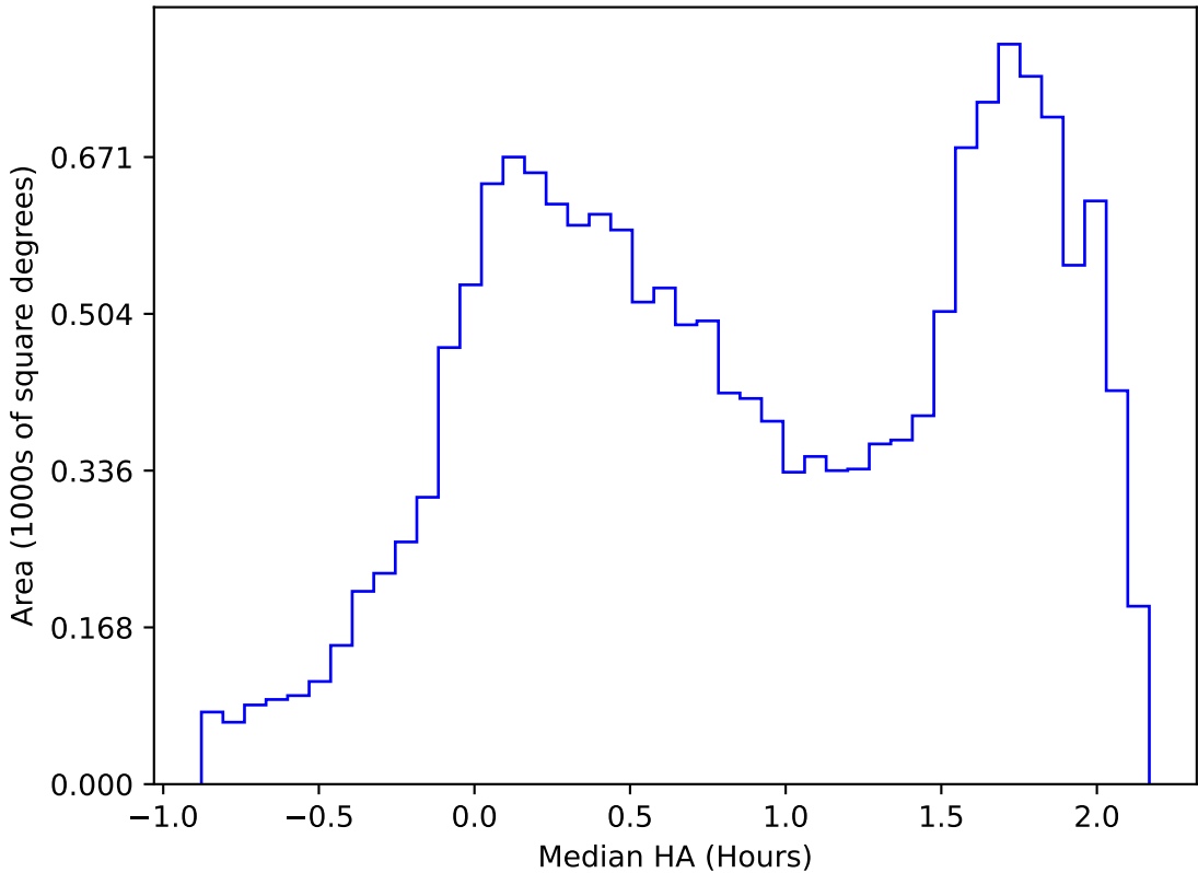
internal_u_expt45_nscale0.9v3.4_10yrs WFD r band: Median HA
