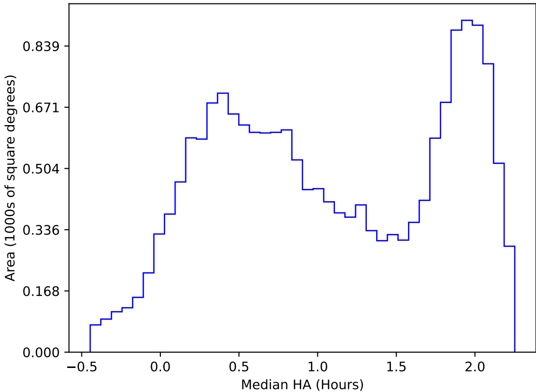
internal_u_expt45_nscale0.9v3.4_10yrs WFD i band: Median HA
