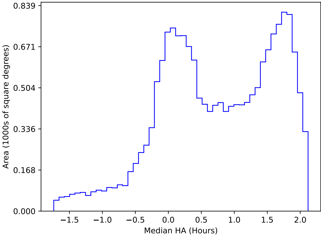
internal_u_expt45_nscale0.9v3.4_10yrs WFD g band: Median HA
