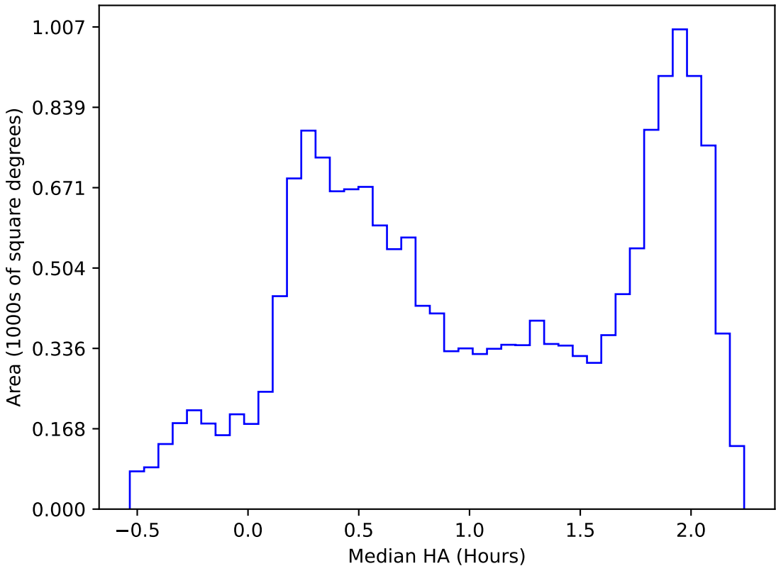
internal_u_expt45_nscale0.9v3.4_10yrs WFD all bands: Median HA
