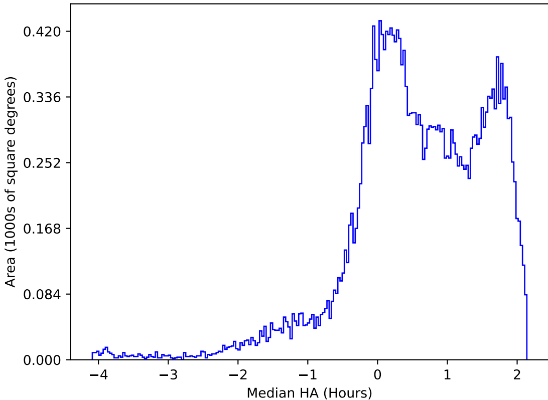
internal_u_expt45_nscale0.9v3.4_10yrs All sky g band: Median HA
