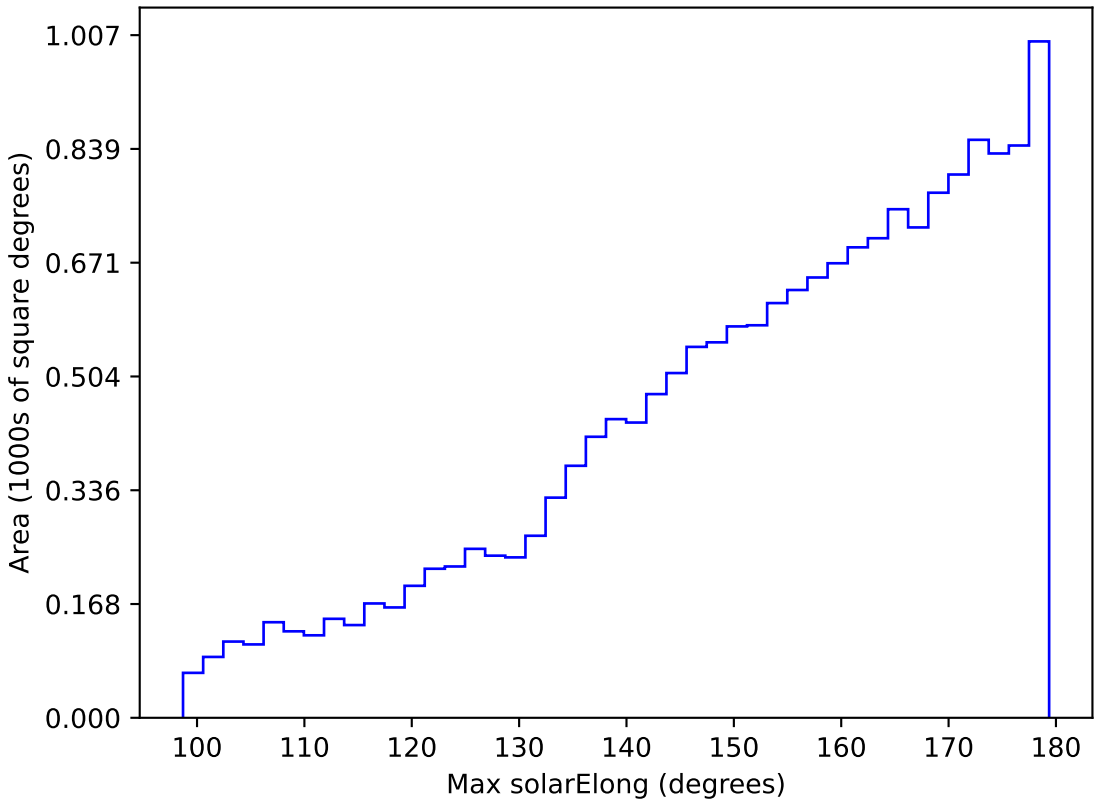
internal_u_expt45_nscale0.9v3.4_10yrs WFD y band: Max solarElong
