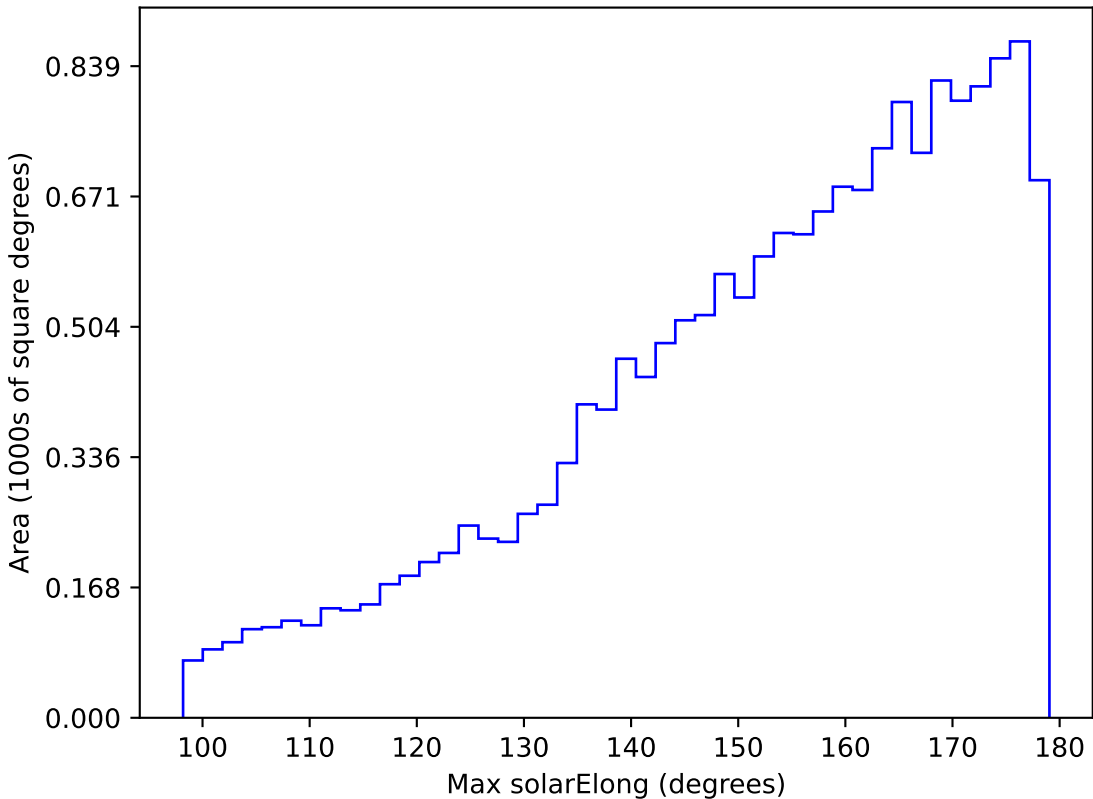
internal_u_expt45_nscale0.9v3.4_10yrs WFD u band: Max solarElong
