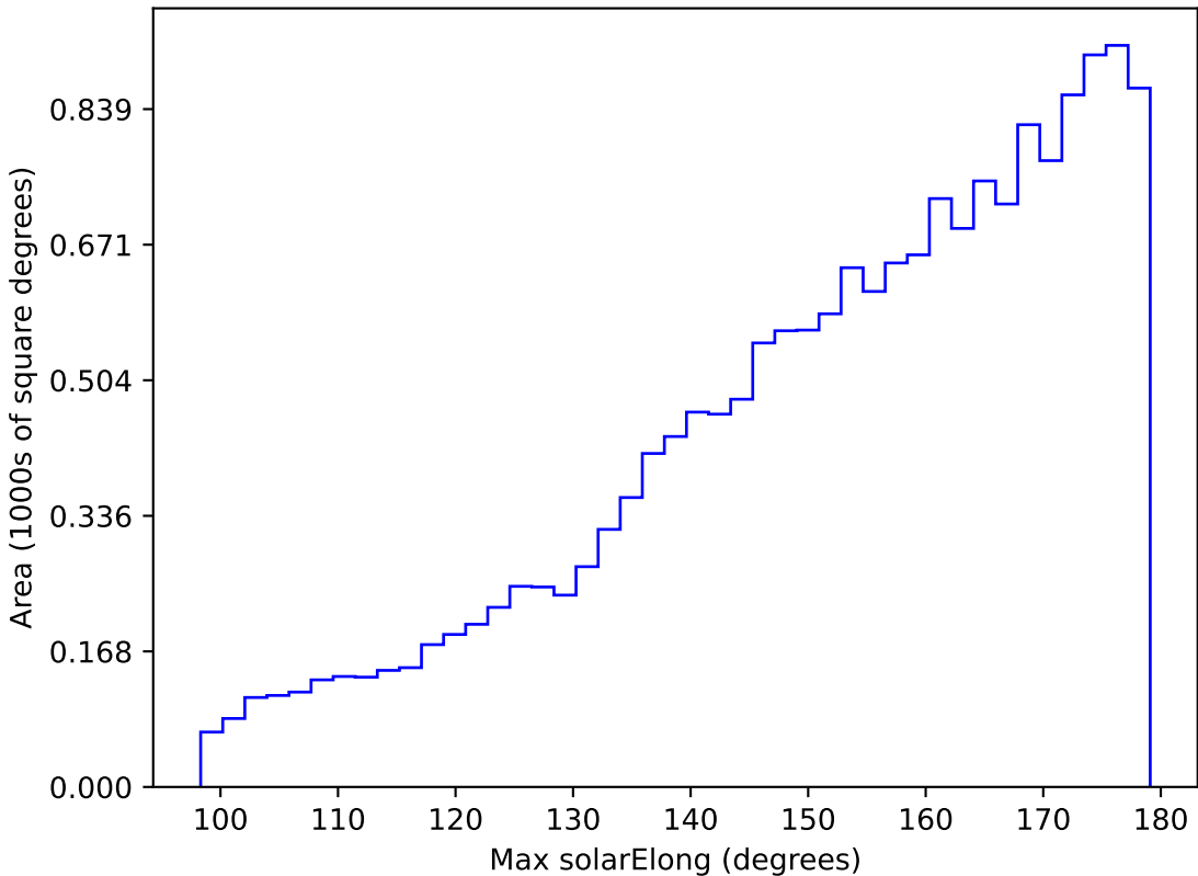
internal_u_expt45_nscale0.9v3.4_10yrs WFD g band: Max solarElong
