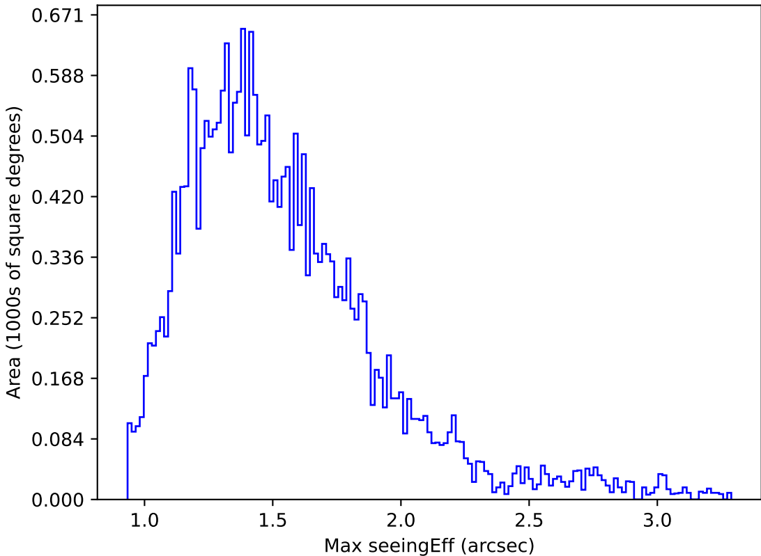
internal_u_expt45_nscale0.9v3.4_10yrs Yr 1 i band: Max seeingEff
