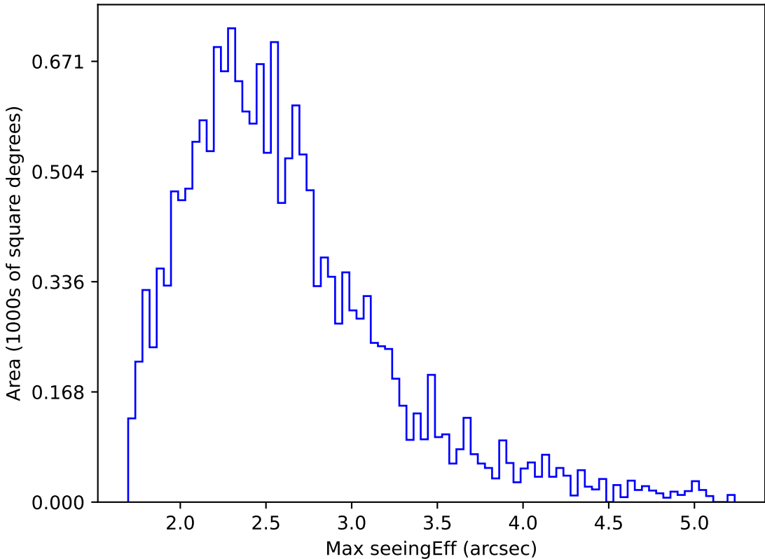
internal_u_expt45_nscale0.9v3.4_10yrs WFD z band: Max seeingEff
