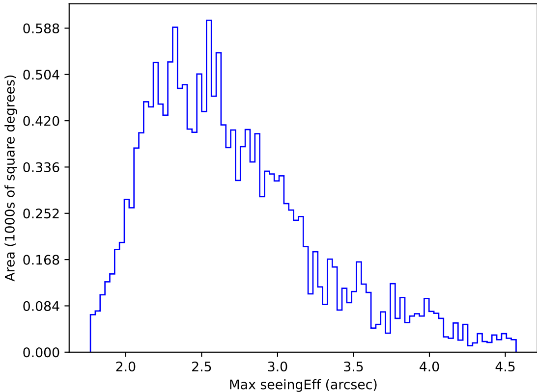
internal_u_expt45_nscale0.9v3.4_10yrs WFD r band: Max seeingEff
