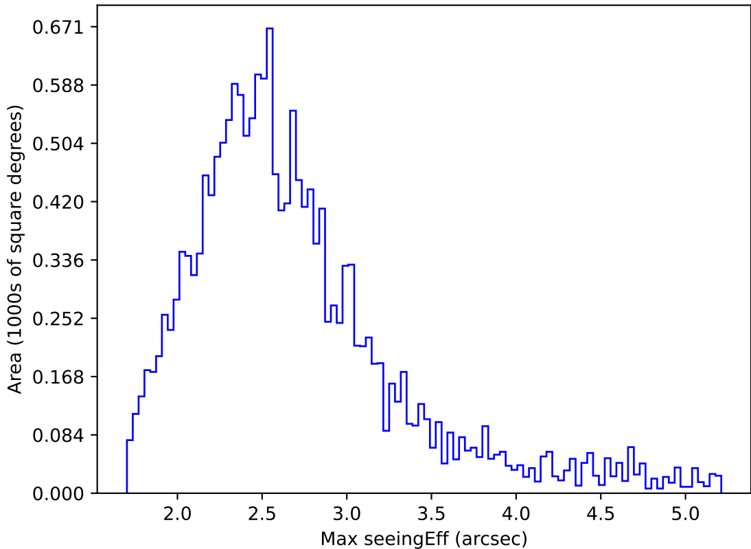
internal_u_expt45_nscale0.9v3.4_10yrs WFD i band: Max seeingEff
