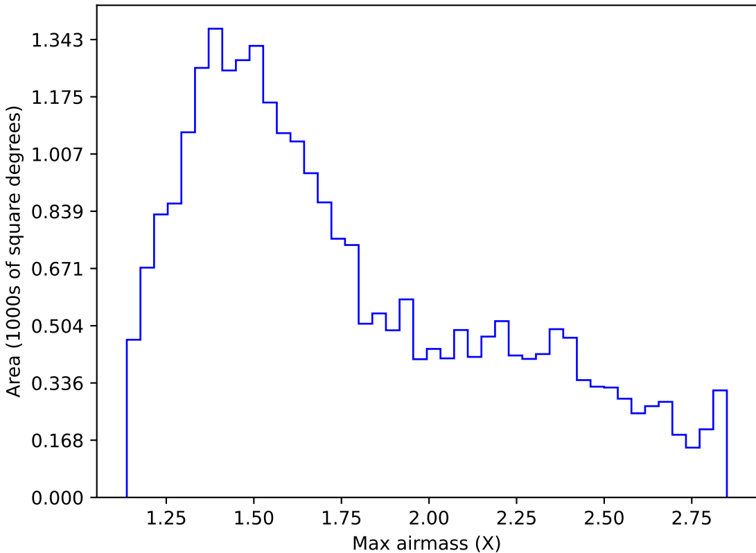
internal_u_expt45_nscale0.9v3.4_10yrs Yr 1 z band: Max airmass
