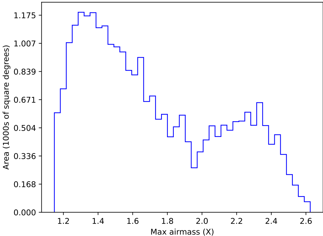
internal_u_expt45_nscale0.9v3.4_10yrs Yr 1 r band: Max airmass
