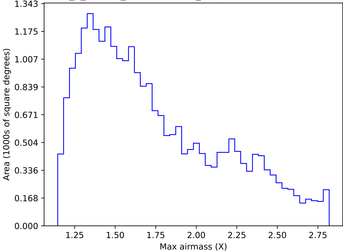
internal_u_expt45_nscale0.9v3.4_10yrs Yr 1 i band: Max airmass
