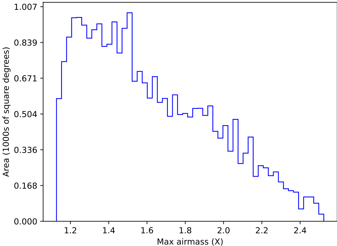
internal_u_expt45_nscale0.9v3.4_10yrs Yr 1 g band: Max airmass
