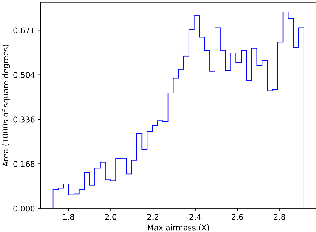
internal_u_expt45_nscale0.9v3.4_10yrs WFD z band: Max airmass
