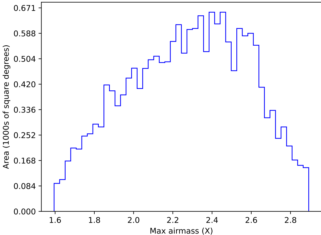
internal_u_expt45_nscale0.9v3.4_10yrs WFD y band: Max airmass
