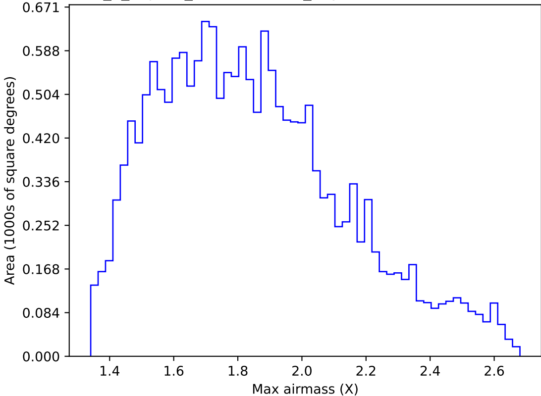
internal_u_expt45_nscale0.9v3.4_10yrs WFD u band: Max airmass
