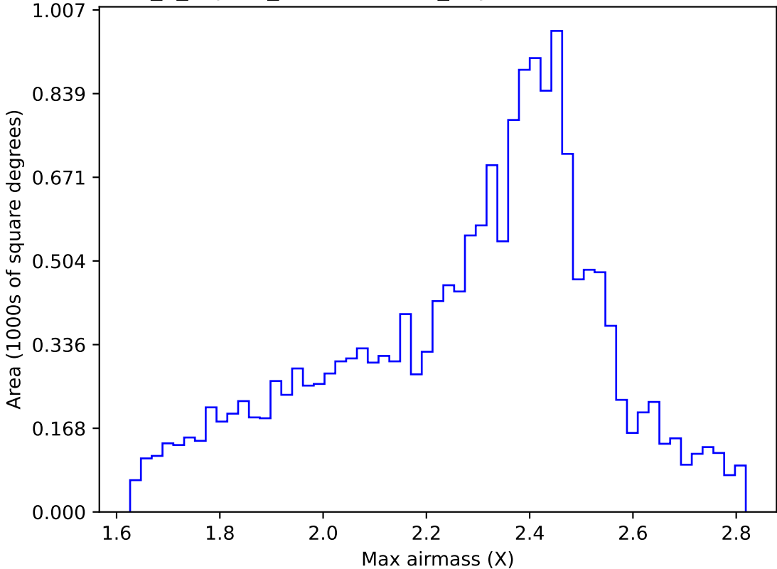
internal_u_expt45_nscale0.9v3.4_10yrs WFD r band: Max airmass
