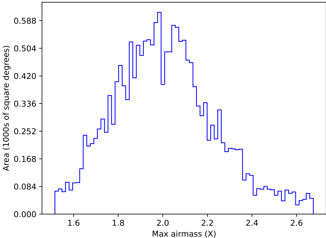
internal_u_expt45_nscale0.9v3.4_10yrs WFD g band: Max airmass
