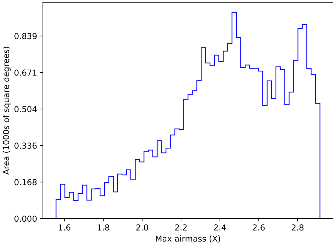
internal_u_expt45_nscale0.9v3.4_10yrs All sky i band: Max airmass
