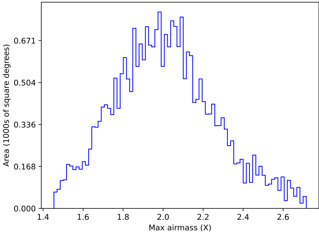
internal_u_expt45_nscale0.9v3.4_10yrs All sky g band: Max airmass
