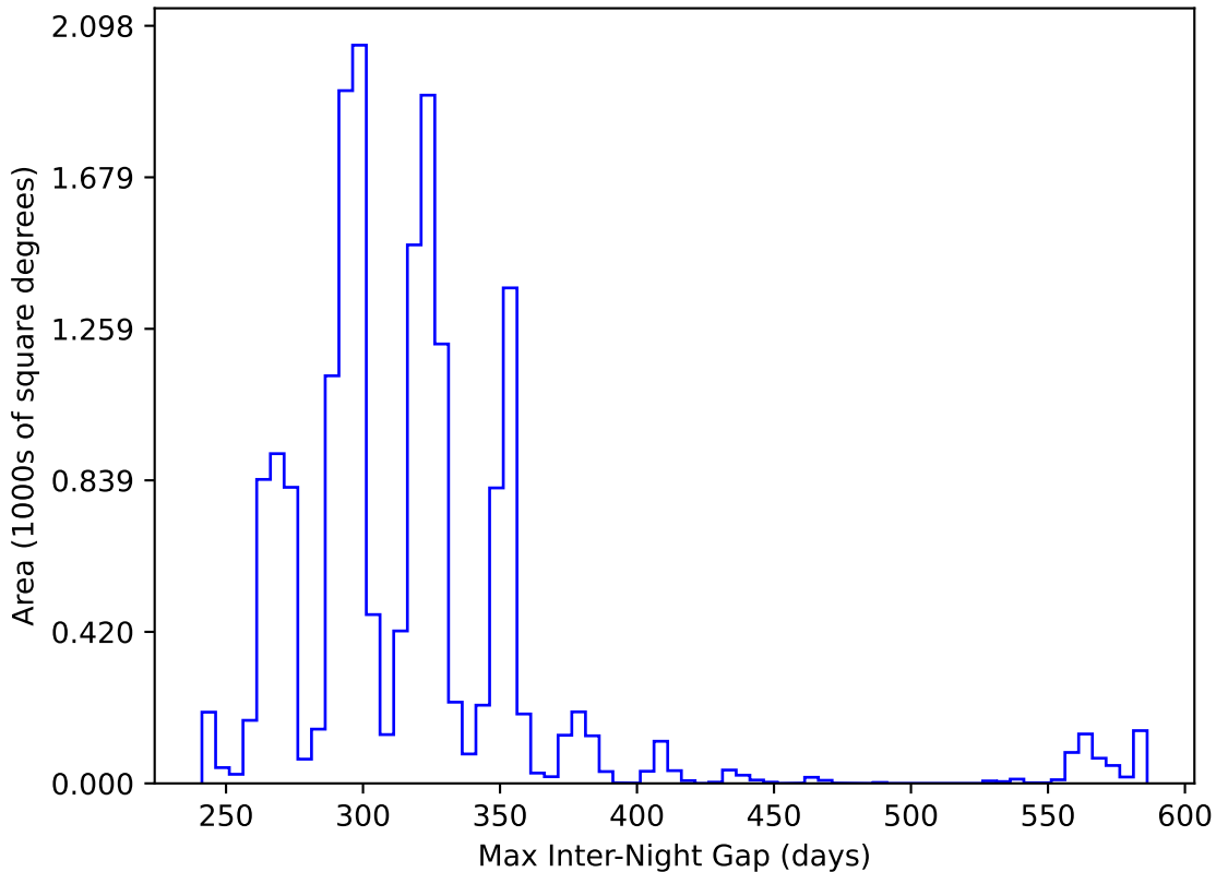
internal_u_expt45_nscale0.9v3.4_10yrs WFD y band: Max Inter-Night Gap
