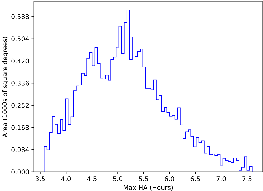
internal_u_expt45_nscale0.9v3.4_10yrs WFD all bands: Max HA
