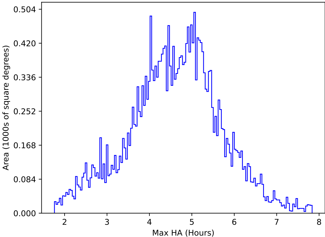
internal_u_expt45_nscale0.9v3.4_10yrs All sky z band: Max HA
