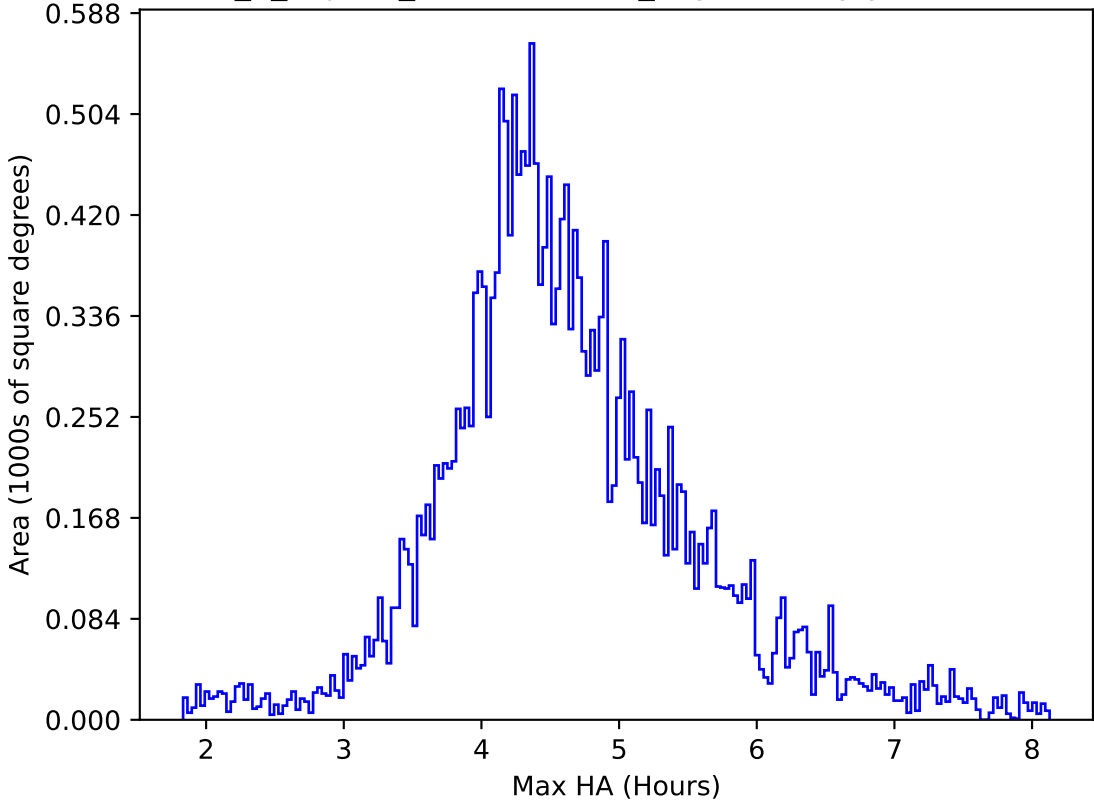
internal_u_expt45_nscale0.9v3.4_10yrs All sky y band: Max HA
