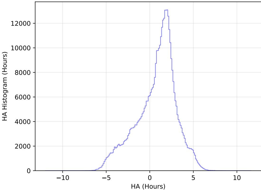
internal_u_expt45_nscale0.9v3.4_10yrs WFD z band: HA Histogram
