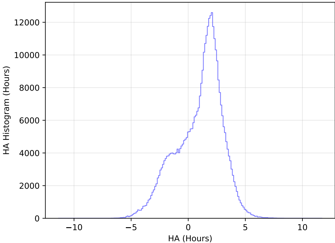
internal_u_expt45_nscale0.9v3.4_10yrs WFD y band: HA Histogram
