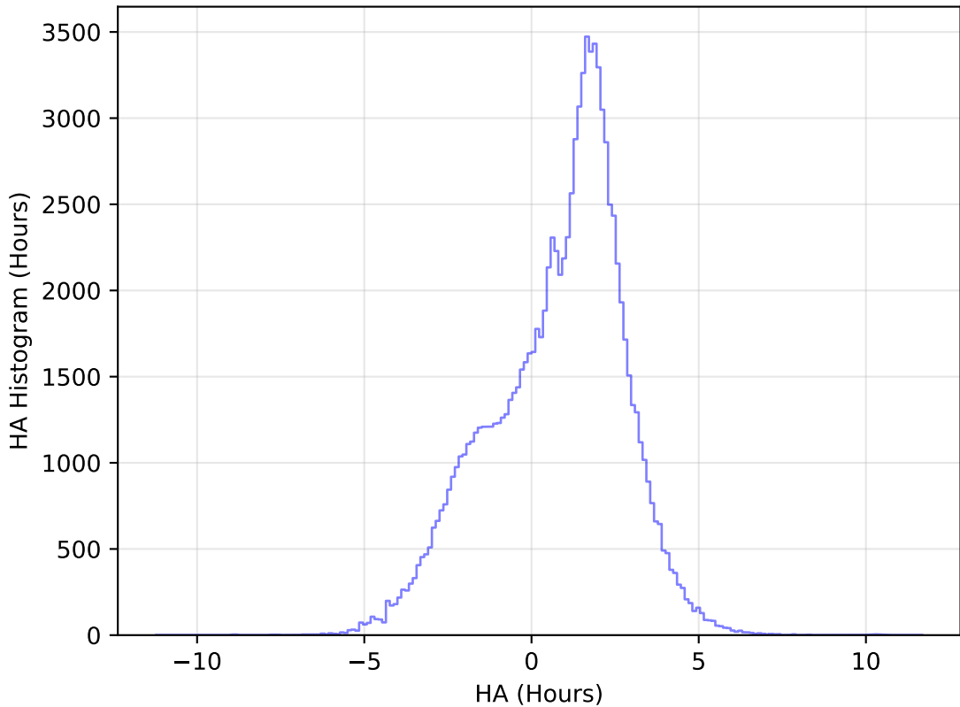
internal_u_expt45_nscale0.9v3.4_10yrs WFD u band: HA Histogram
