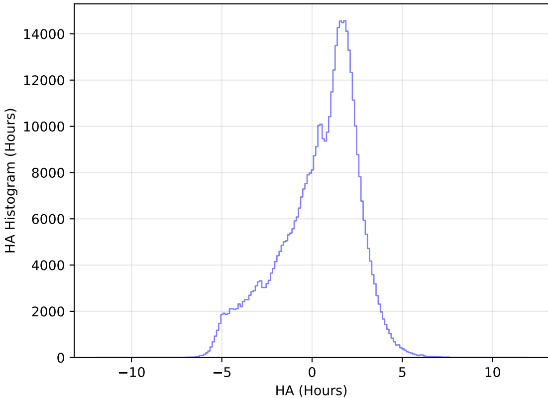
internal_u_expt45_nscale0.9v3.4_10yrs WFD r band: HA Histogram
