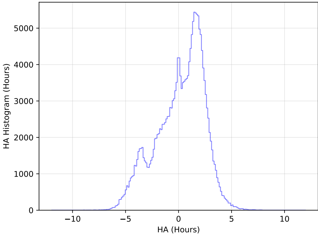
internal_u_expt45_nscale0.9v3.4_10yrs WFD g band: HA Histogram
