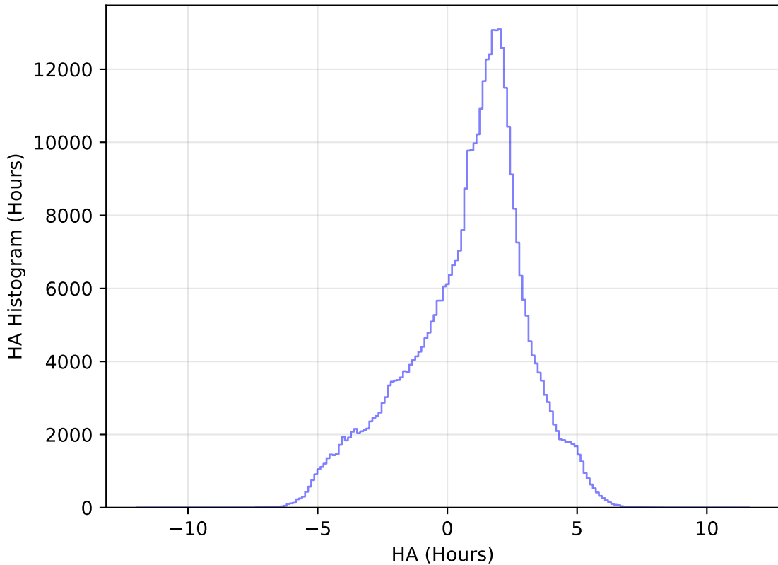
internal_u_expt45_nscale0.9v3.4_10yrs All sky z band: HA Histogram
