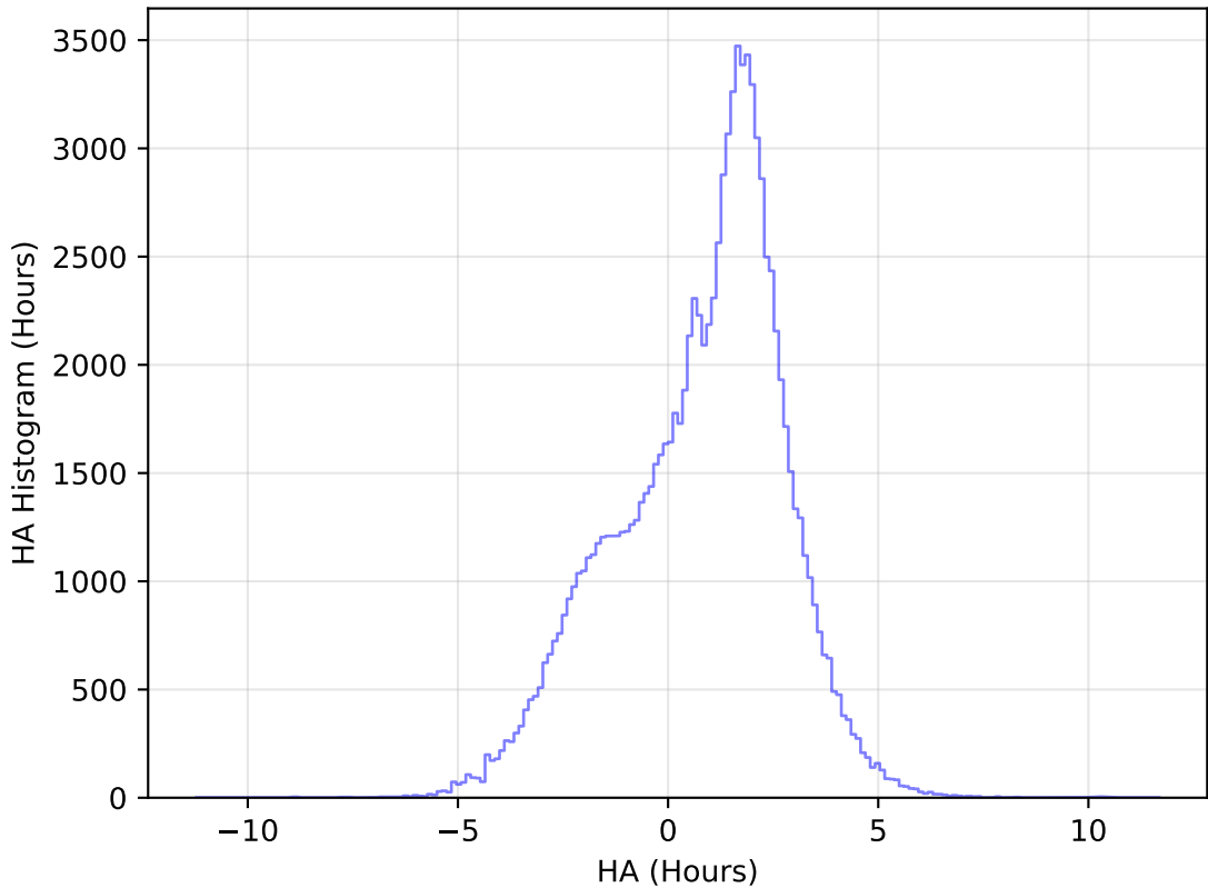
internal_u_expt45_nscale0.9v3.4_10yrs All sky u band: HA Histogram
