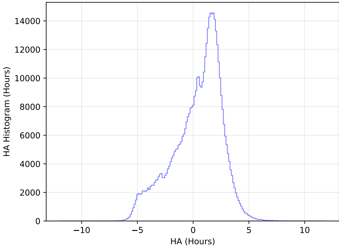
internal_u_expt45_nscale0.9v3.4_10yrs All sky r band: HA Histogram
