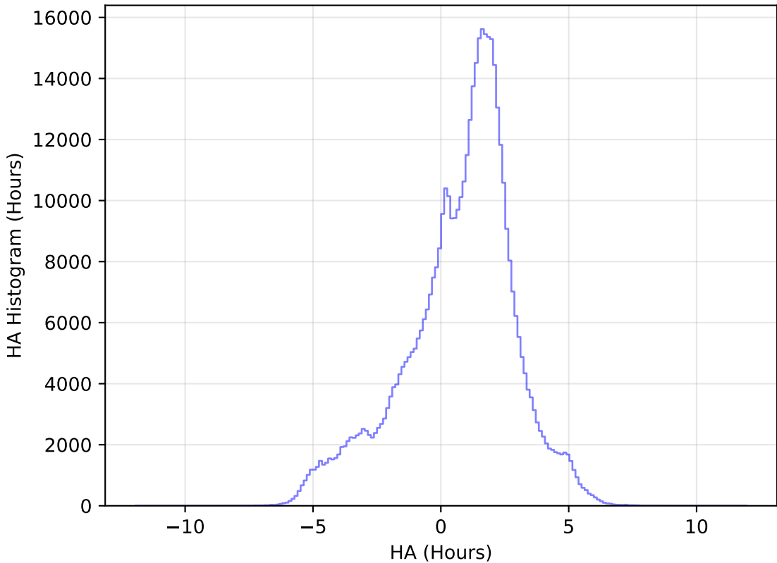
internal_u_expt45_nscale0.9v3.4_10yrs All sky i band: HA Histogram
