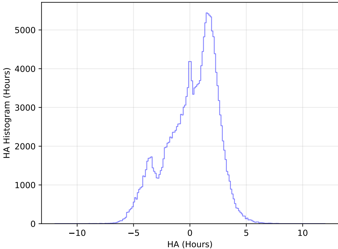
internal_u_expt45_nscale0.9v3.4_10yrs All sky g band: HA Histogram
