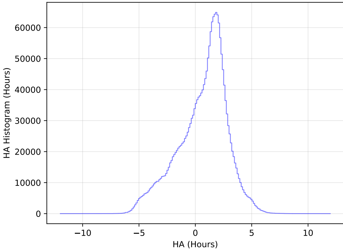
internal_u_expt45_nscale0.9v3.4_10yrs All sky all bands: HA Histogram
