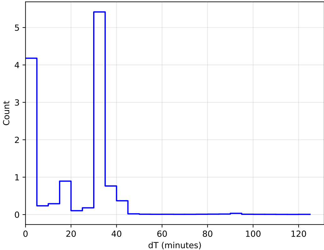
internal_u_expt45_nscale0.9v3.4_10yrs All sky: DeltaT Histogram
