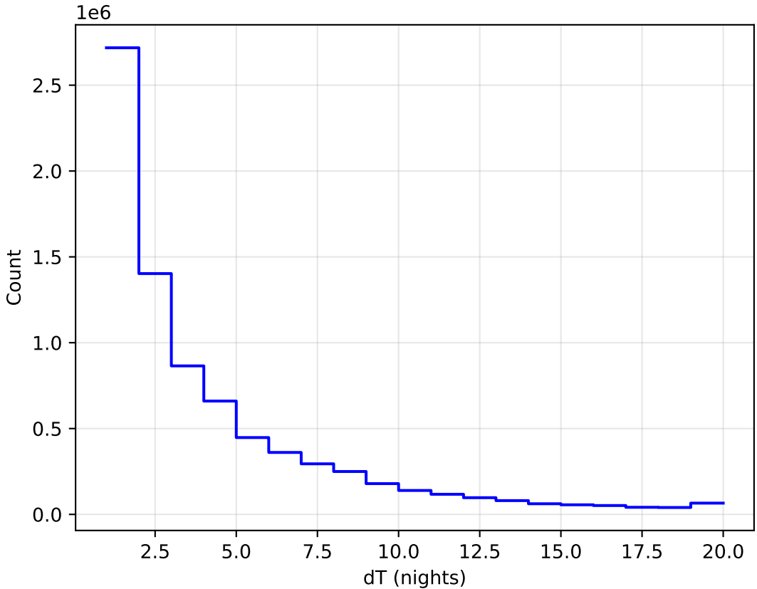
internal_u_expt45_nscale0.9v3.4_10yrs WFD all bands: DeltaNight Histogram
