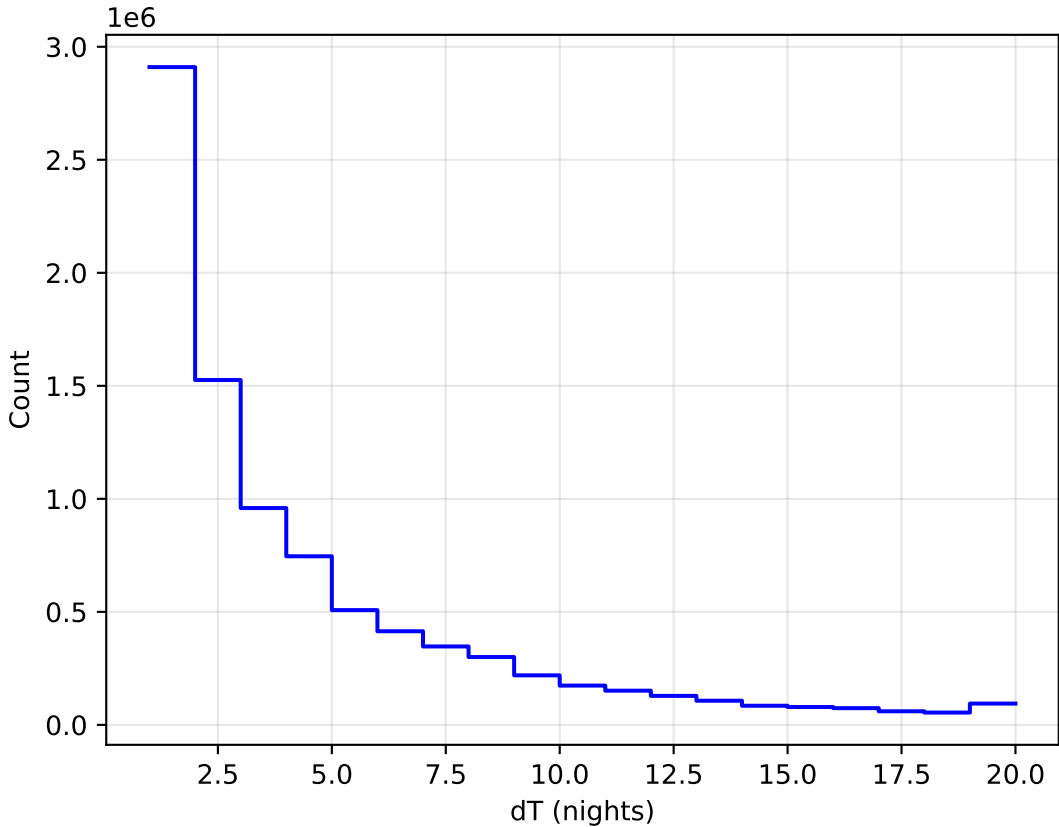
internal_u_expt45_nscale0.9v3.4_10yrs All sky all bands: DeltaNight Histogram
