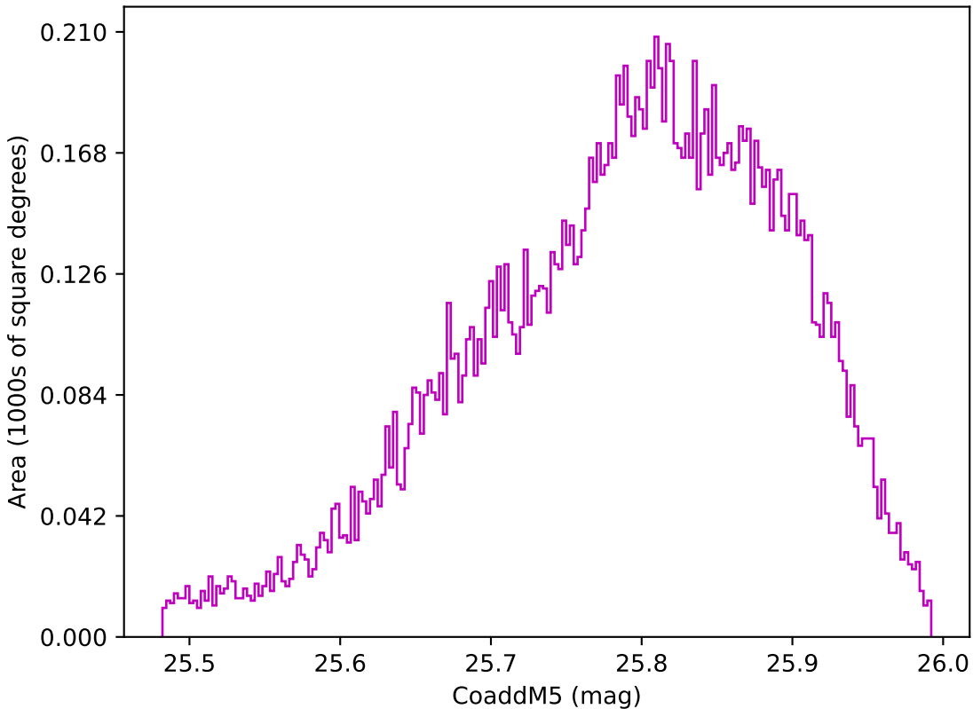
internal_u_expt45_nscale0.9v3.4_10yrs WFD z band: CoaddM5
