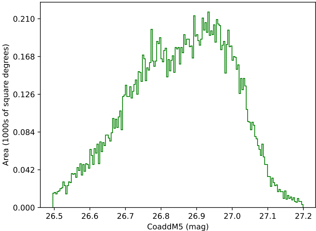
internal_u_expt45_nscale0.9v3.4_10yrs WFD g band: CoaddM5
