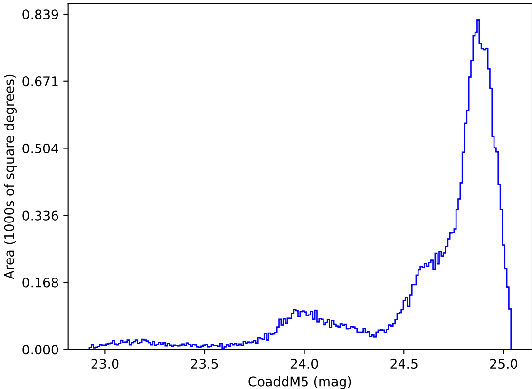
internal_u_expt45_nscale0.9v3.4_10yrs All sky y band: CoaddM5
