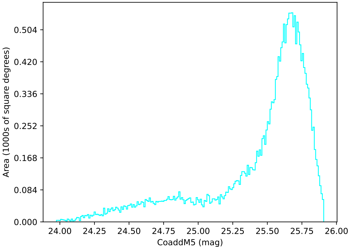
internal_u_expt45_nscale0.9v3.4_10yrs All sky u band: CoaddM5
