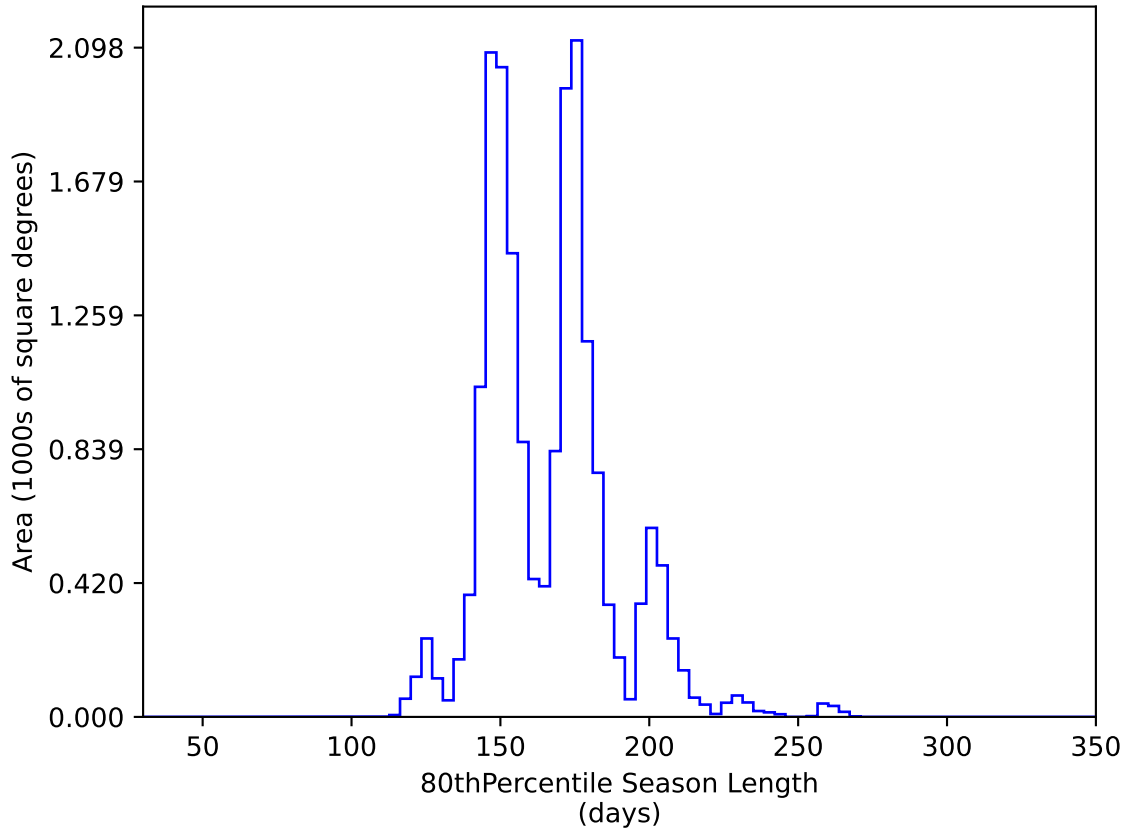
internal_u_expt45_nscale0.9v3.4_10yrs WFD y band: 80thPercentile Season Length
