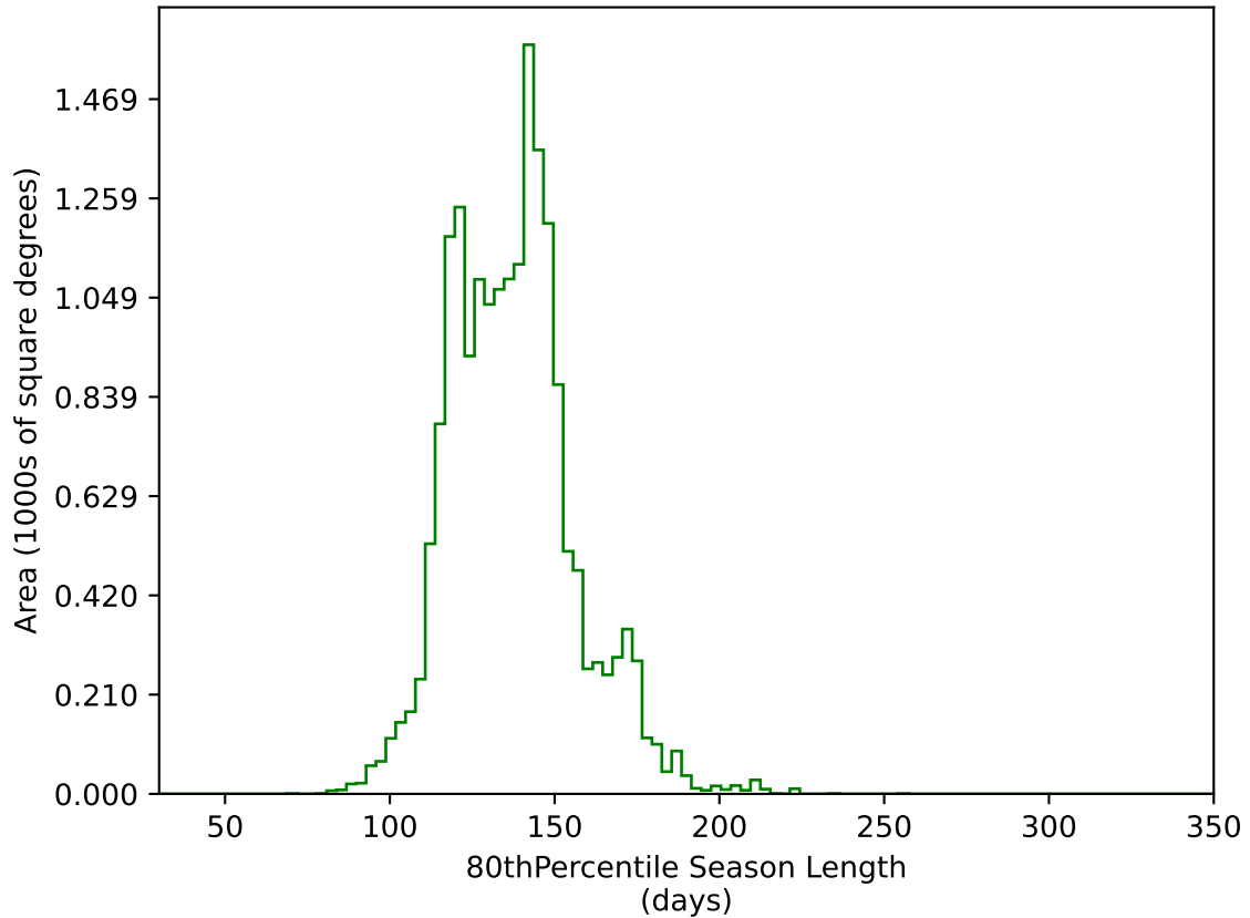
internal_u_expt45_nscale0.9v3.4_10yrs WFD g band: 80thPercentile Season Length
