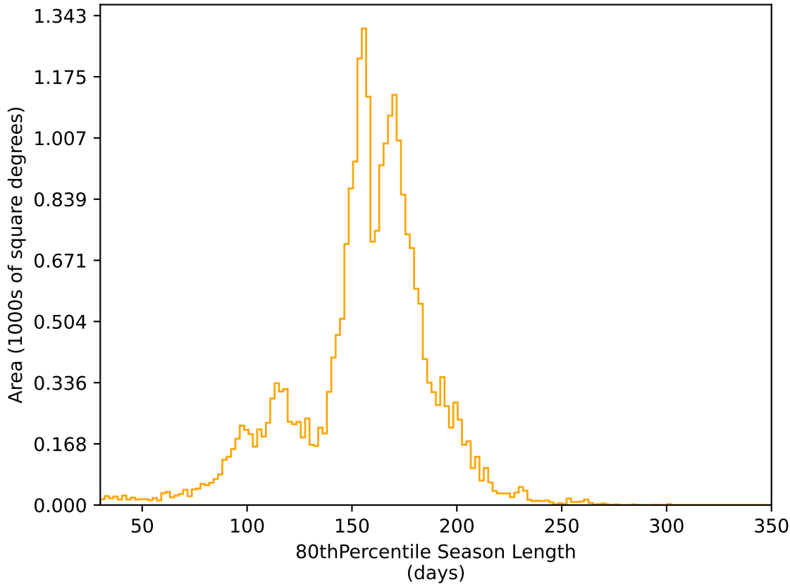
internal_u_expt45_nscale0.9v3.4_10yrs All sky r band: 80thPercentile Season Length
