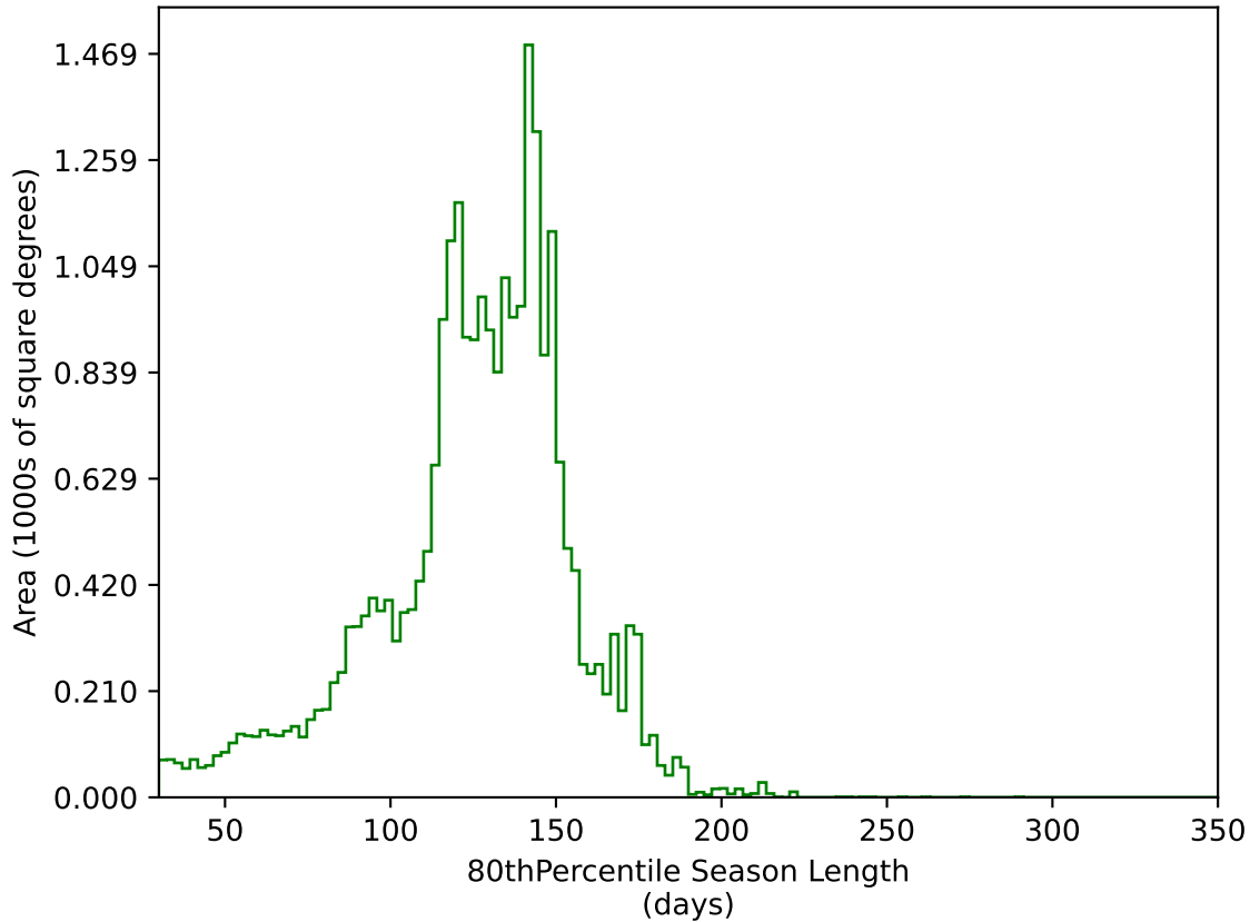
internal_u_expt45_nscale0.9v3.4_10yrs All sky g band: 80thPercentile Season Length
